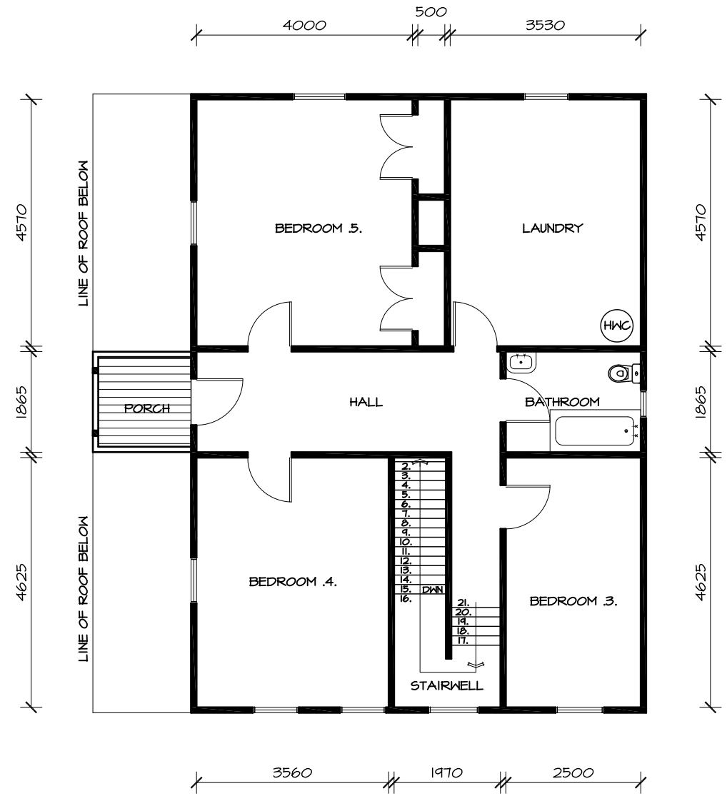
EXISTING FIRST FLOOR PLAN SCALE 1:100 @ A3
