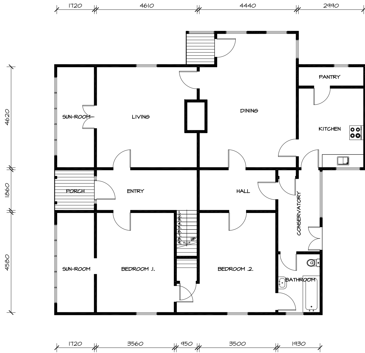
EXISTING GROUND FLOOR PLAN SCALE 1:100 @ A3
