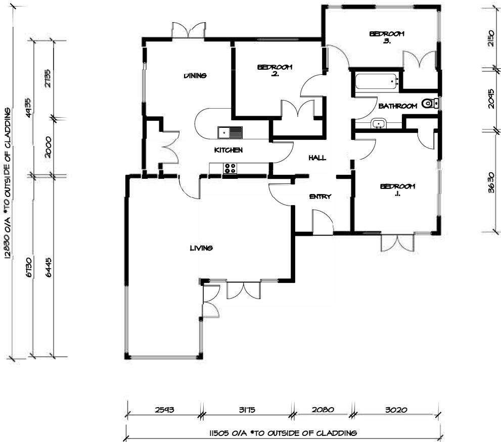
EXISTING FLOOR PLAN SCALE 1:100 • A3
